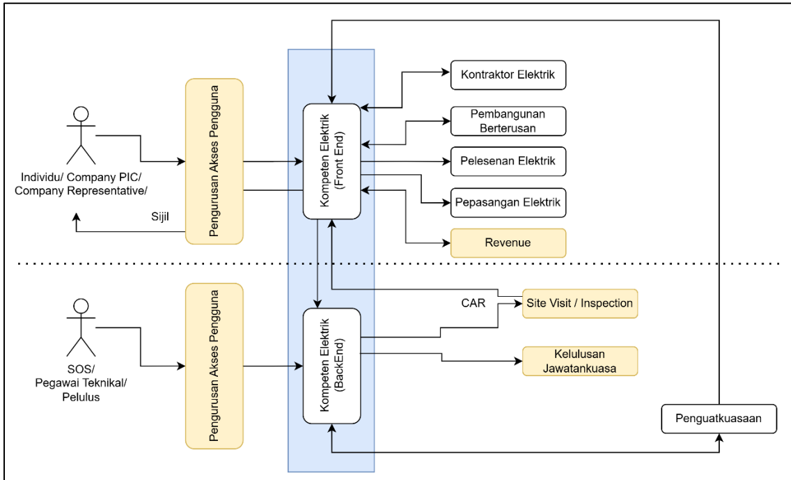
Rajah 8: Integrasi Modul RG-KE
