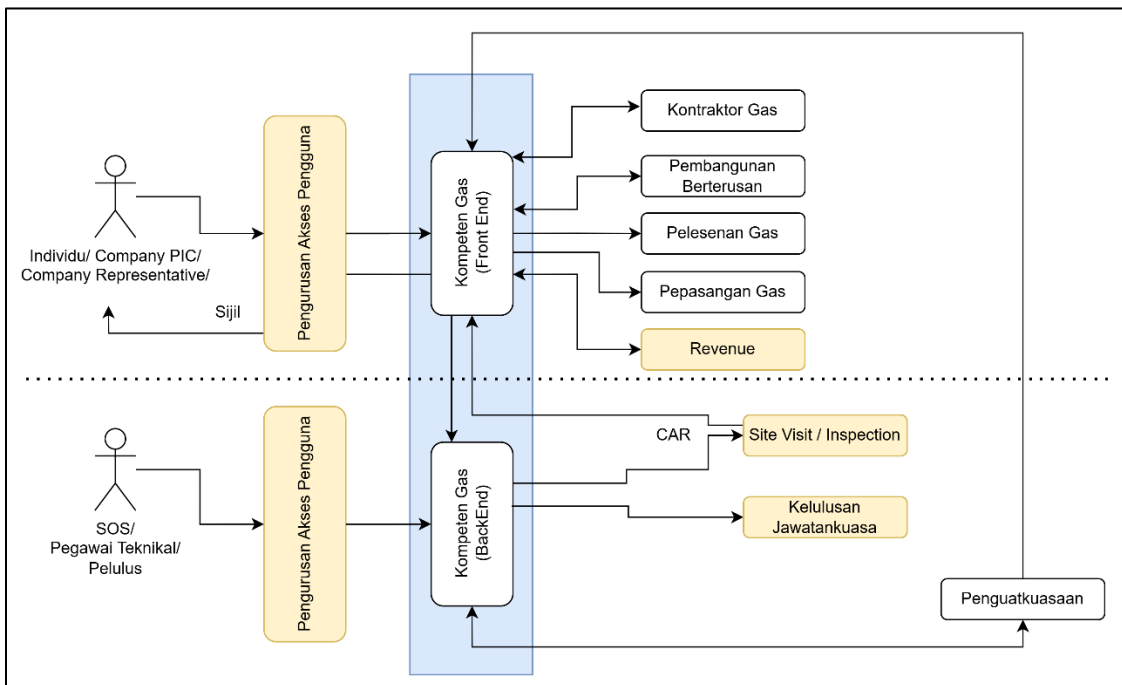
Rajah 9: Integrasi Modul RG-KG
