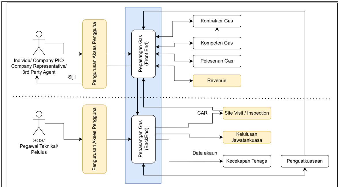
Rajah 4: Integrasi Modul LC - PG
