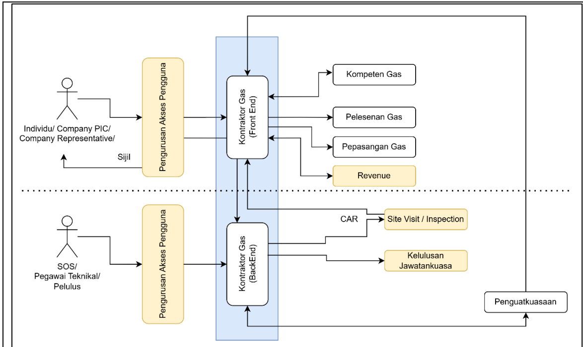
Rajah 11: Integrasi Modul RG-CG
